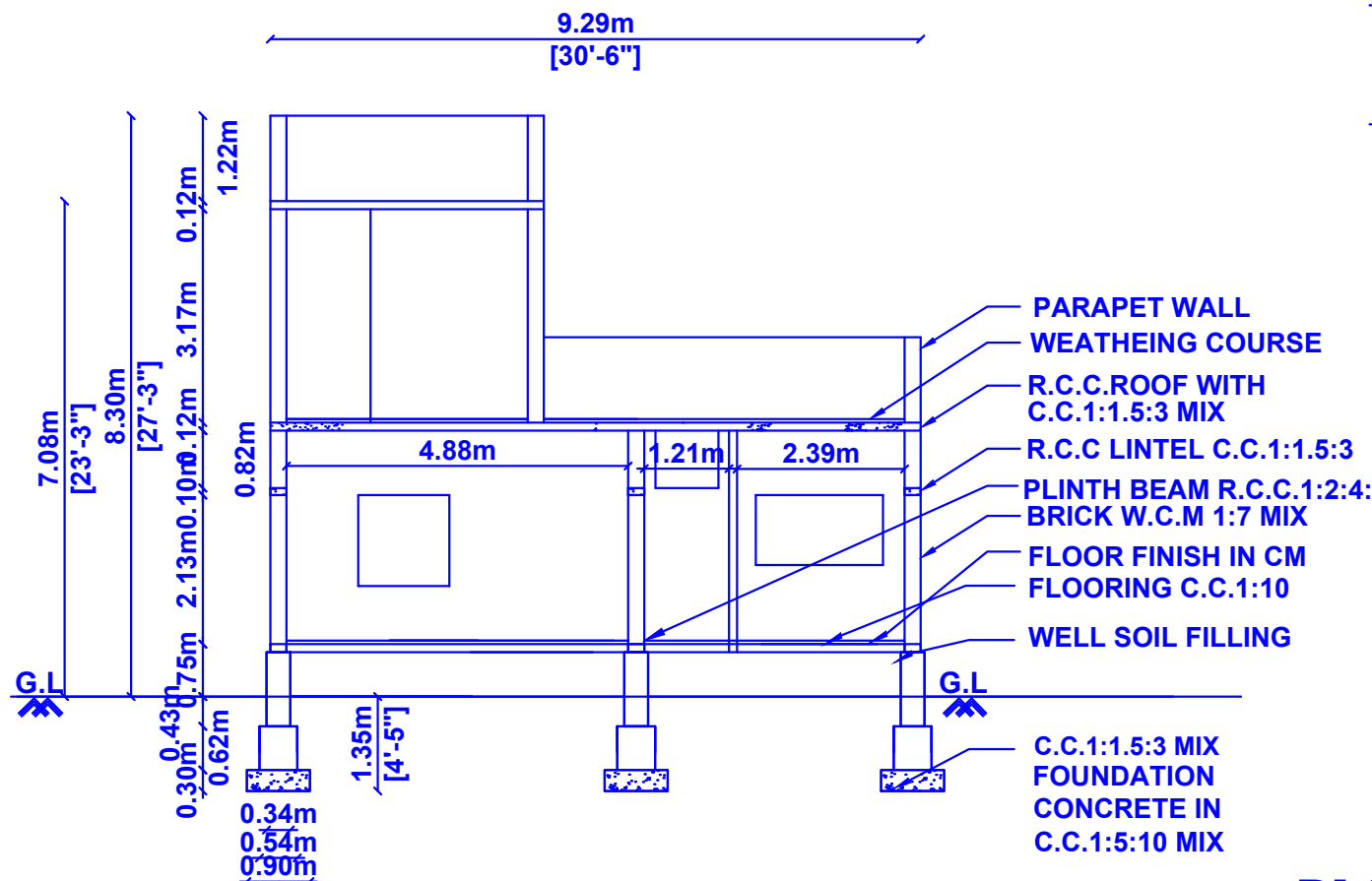
SECTION ON G1G2'
