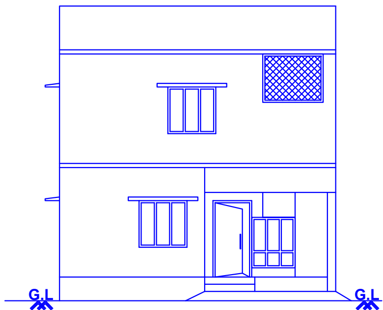
FRONT ELEVATION
