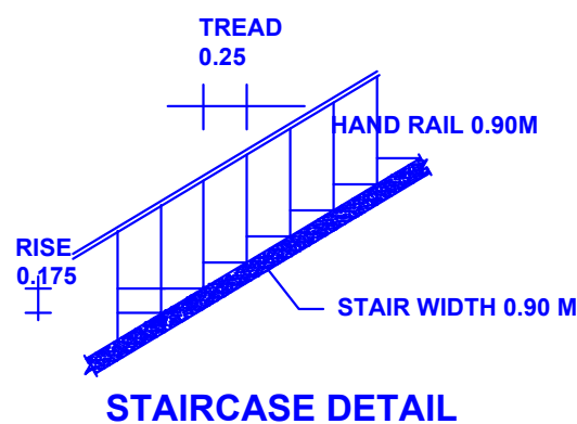
STAIRCASE DETAIL
