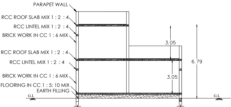
SECTION ON AB & ( HALF ELEVATION)
