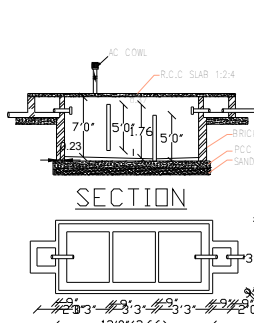
PLAN SEPTIC TANK DETAILS
