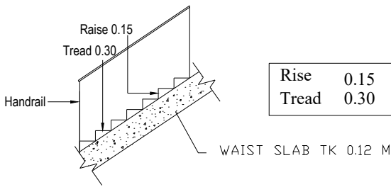
STAIRCASE DETAIL
