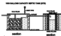
SECTION ON - A B
