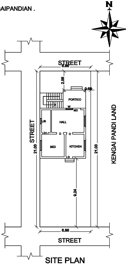
SITE PLAN
