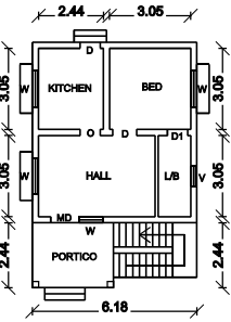
G.F. PLAN
