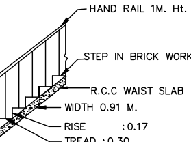
STAIR DETAIL
