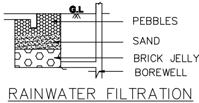
RAINWATER FILTRATION
