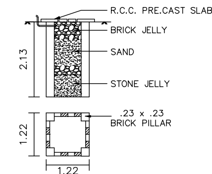
PLAN & SECTION OF RAIN WATER COLLECTION WELL
