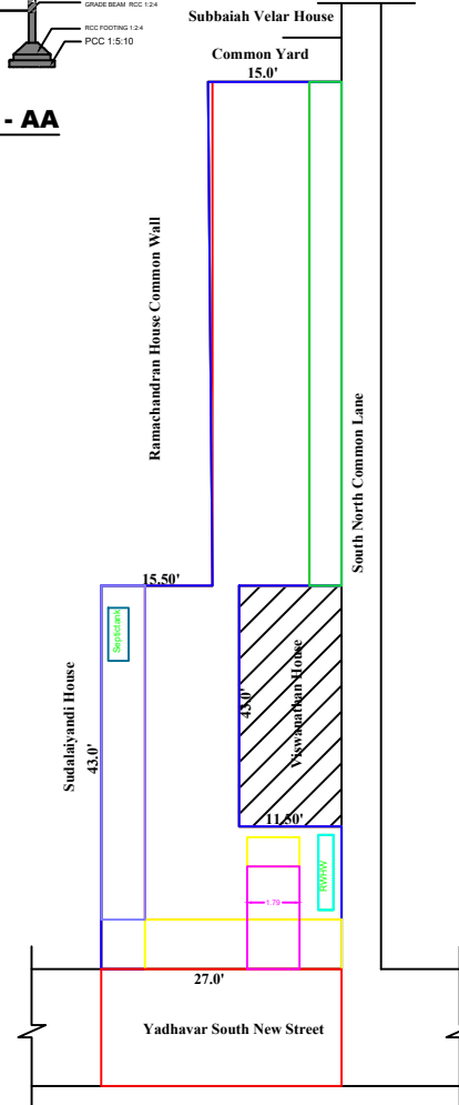
SITE PLAN
