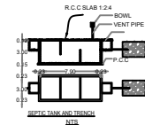
SECTION ON - AA
