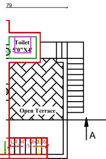
PRO.FIRST FLOOR PLAN
