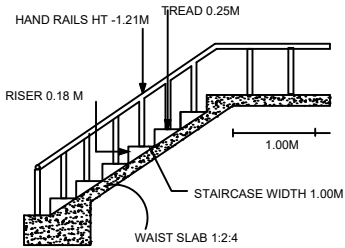
STAIRCASE DETAILS
