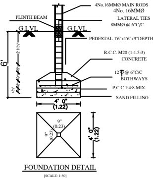
FOUNDATION DETAIL
