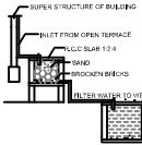
DETAILS OF FILTER BED & WELL
