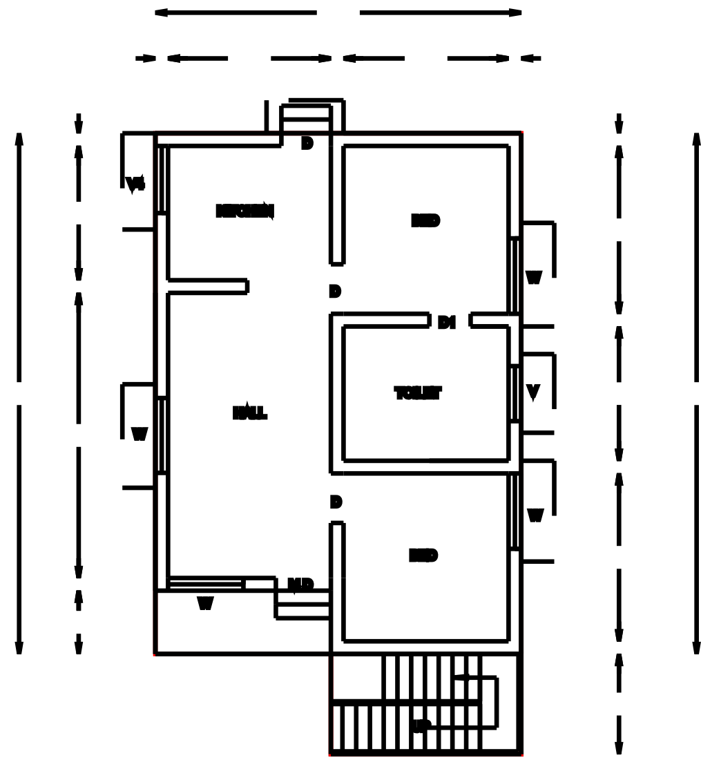
PLAN
