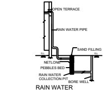
RAIN WATER
