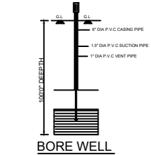
BORE WELL
