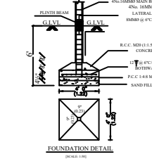
FOUNDATION DETAIL
