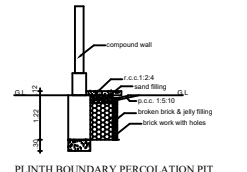
PLINTH BOUNDARY PERCOLATION PIT
