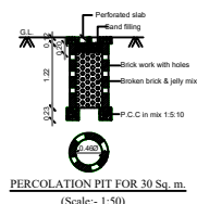
PERCOLATION PIT FOR 30 Sq. m. (Scale:- 1:50)
