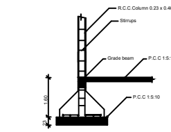
COLUMN DETAIL
