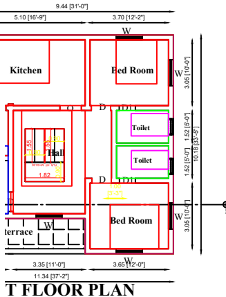
T FLOOR PLAN
