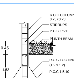
COLUMN DETAILS
