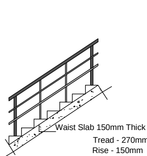
STAIR CASE DETAIL
