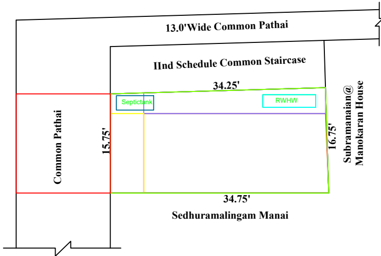
SITE PLAN
