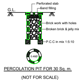
RAINWATER HARVESTING
