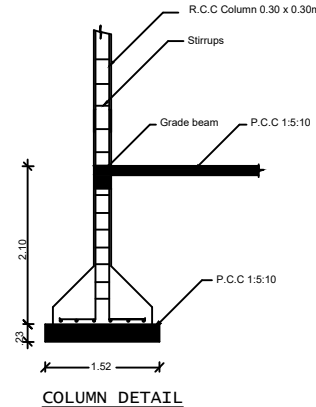
COLUMN DETAIL
