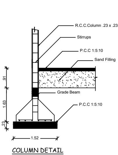
COLUMN DETAIL
