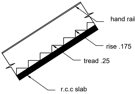
STAIR
