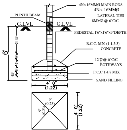
FOUNDATION DETAIL (SCALE: 1:50)
