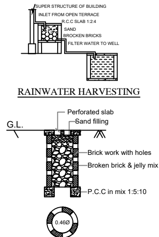
PERCOLATION PIT FOR 30 Sq. m. (NOT FOR SCALE)
