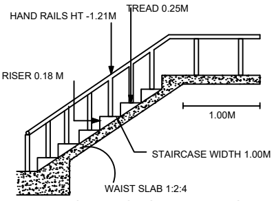
STAIRCASE DETAILS
