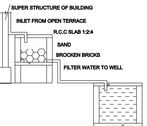
Rainwater harvesting
