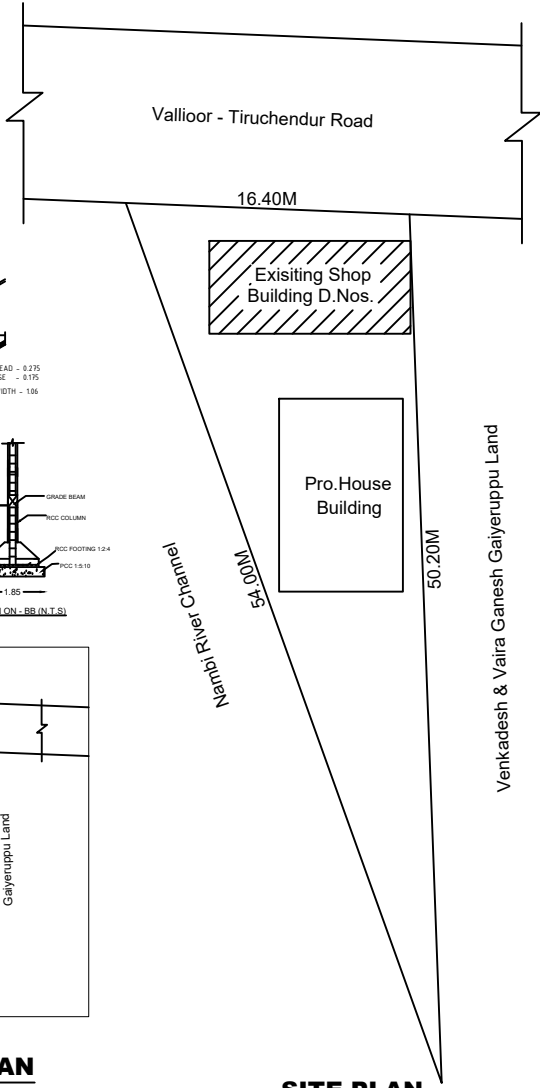
SITE PLAN
