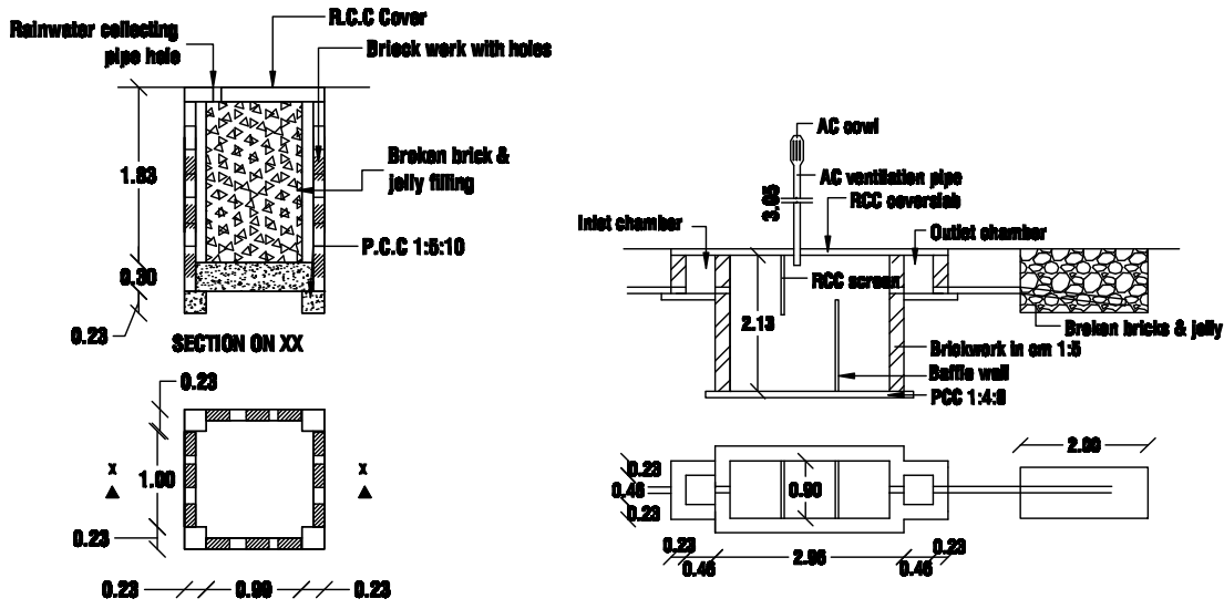
SEPTICTANK DETAILS
