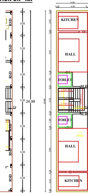
EXG.FIRST FLOOR PLAN
