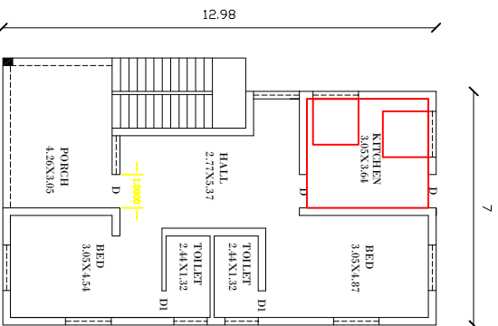
GROUND FLOOR PLAN(1:100)
