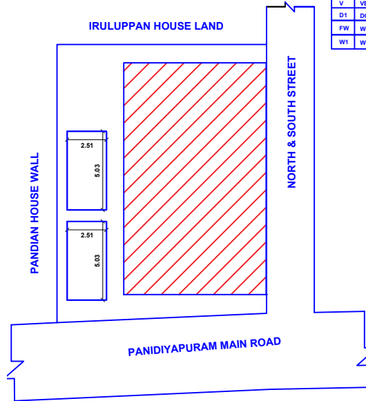
SITE PLAN SCALE 1CM:1METER
