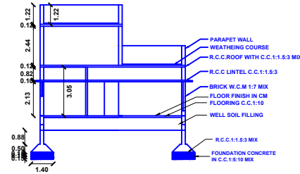
SECTION ON G1G2"
