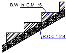
STAIRCASE
