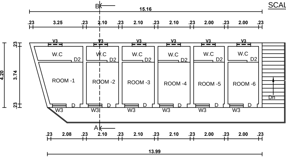
FF PLAN
