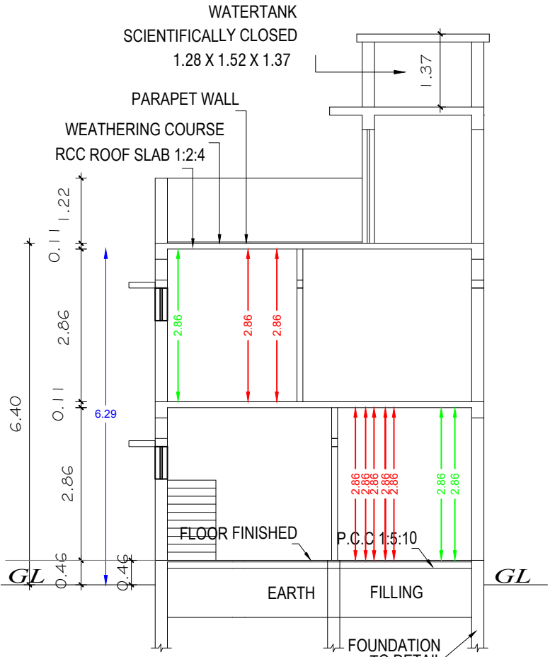
SECTION "A-B"
