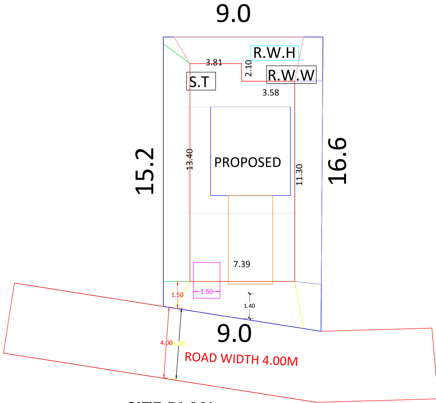
SITE PLAN
