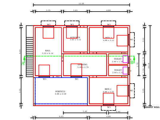
PRO. GROUND FLOOR PLAN
