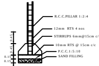
COLUMN DETAILS SCALE 1:50
