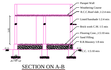
SECTION ON A-B
