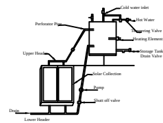
Details Of Solar Water Heater (NTS)
