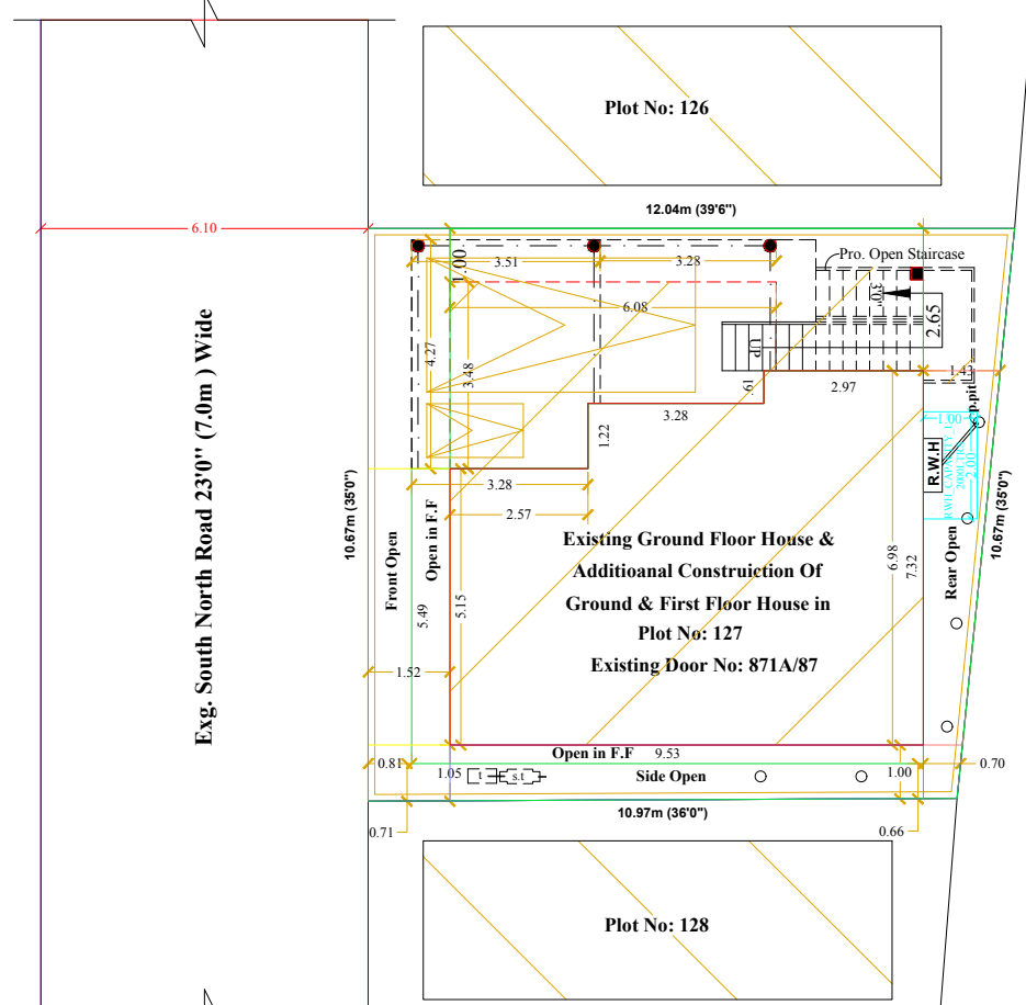
SITE PLAN
