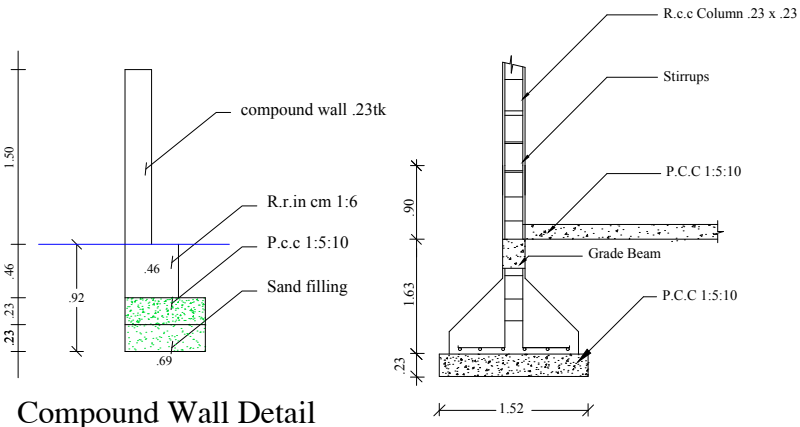
COLUMN DETAIL
