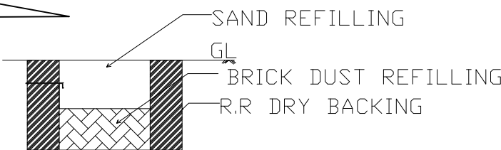
DETAILS OF RAIN WATER HARVESTING
