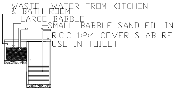
RECYCLING OF WASTE WATER FROM KITCHEN & BATHROOM
