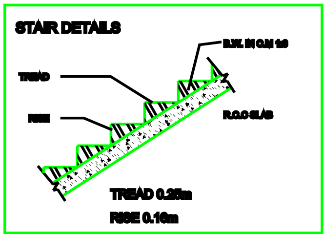
STAIR DETAILS
