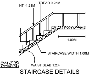
STAIRCASE DETAILS
