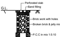
RAINWATER HARVESTING
