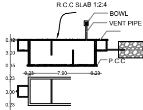
SEPTIC TANK AND FILTER BED
