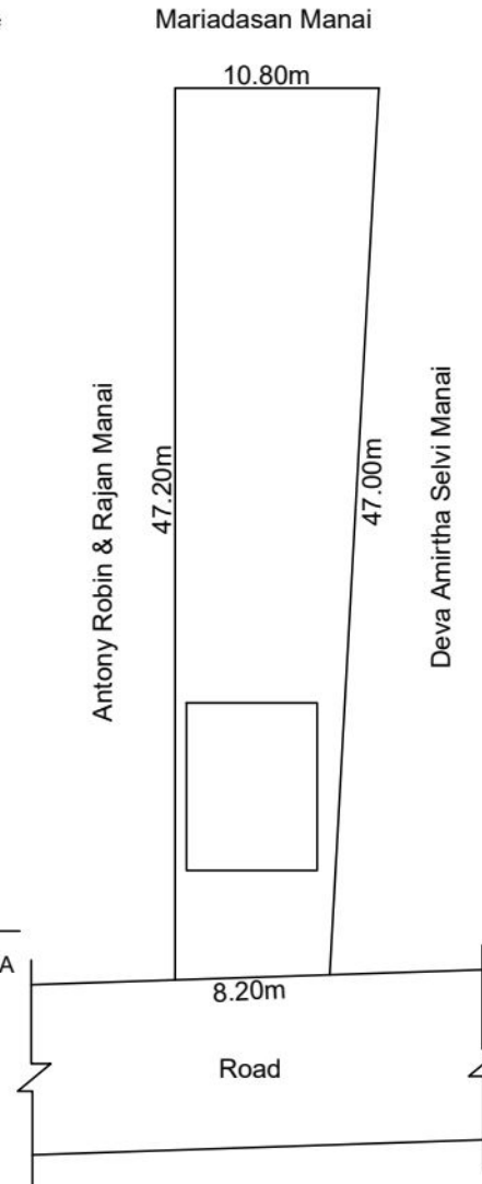
SITE PLAN
