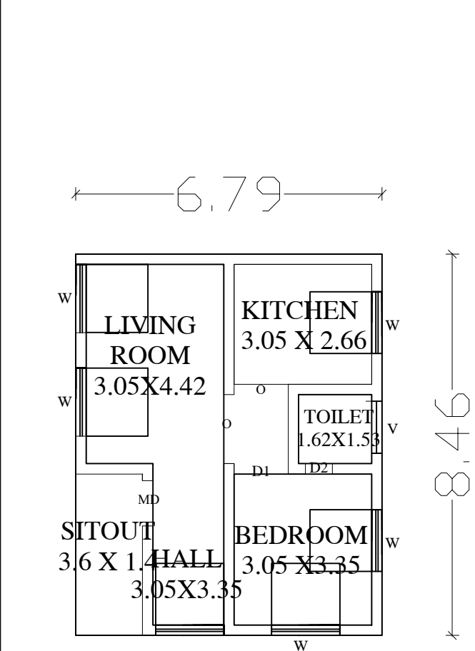
GROUND PLAN
