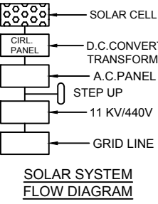
SOLAR SYSTEM FLOW DIAGRAM
