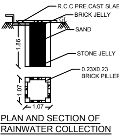
PLAN AND SECTION OF RAINWATER COLLECTION WELL
