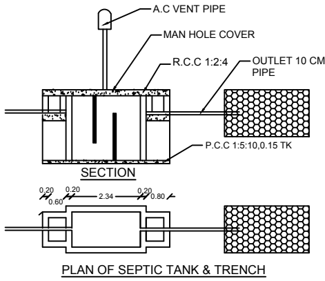
PLAN OF SEPTIC TANK & TRENCH
