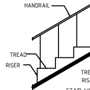
STAIRCASE DETAILS
