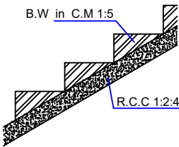
STAIRCASE
