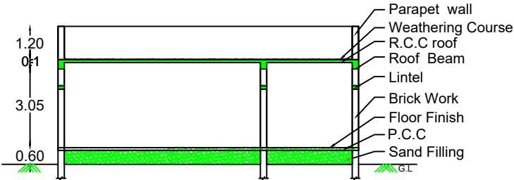
SECTION AB
