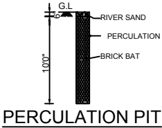
PERCOLATION PIT
