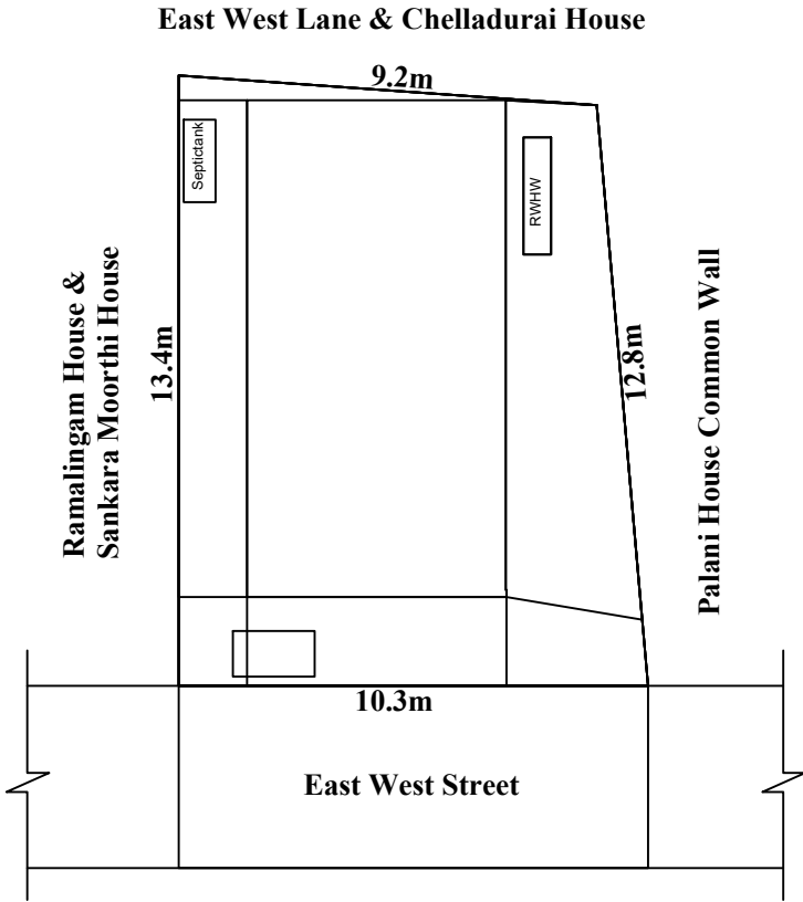
SITE PLAN
