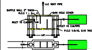
Septic Tank
