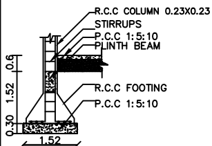
COLOUMN DETAILS
