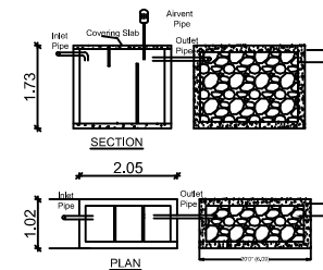
DETAILS OF SEPTIC TANK & DISPERSION TRENCH
