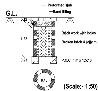
RAIN WATER COLLECTION WELL
