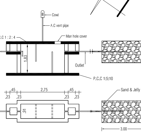
SEPTIC TANK AND TRENCH
