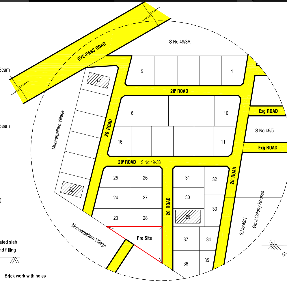
TOPO PLAN
