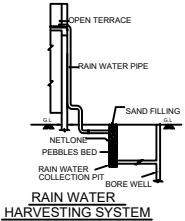
SECTION-AB
