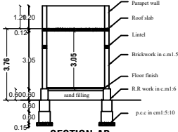
SECTION-AB
