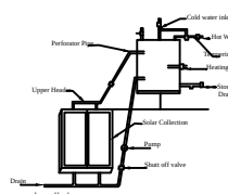
Details Of Solar Water Heater (NTS)
