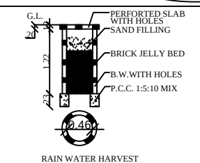
RAIN WATER HARVEST
