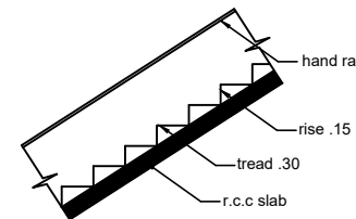
STAIR
