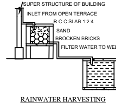
RAINWATER HARVESTING
