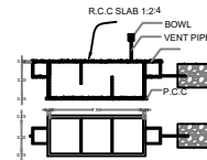
SEPTIC TANK AND TRENCH NTS
